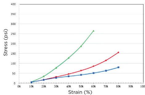
Stress Vs. Strain of GPE100HI-HI/HO/HU (1.0mm thick) with Step Application of Strain (@ Temp=25-29°C; Rate of Strain = 0.01 inch/min between each step application of strain; stress measurement time interval of 2 min for each step application of strain)
