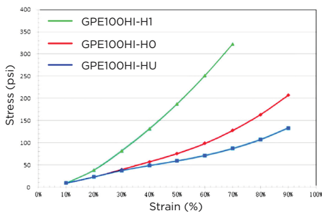
Stress Vs. Strain of GPE100HI-HI/HO/HU (1.0mm thick) with Constant Rate of Strain (@ Temp=25-29°C; Constant Rate of Strain = 0.01 inch/min)
