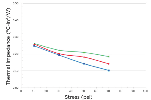
Thermal Impedance Vs. Stress of GPE100HI-HI/HO/HU (1.0mm thick) (at Temp=60°C; Step application of pressure 10, 30, 50, 70 psi; ASTM D5470 modified)
